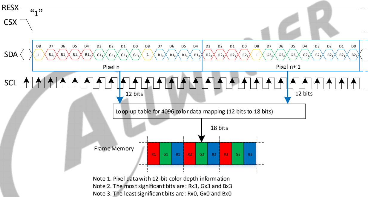
Figure 9-48 RGB444 3-Line Interface Transmit Video Format
