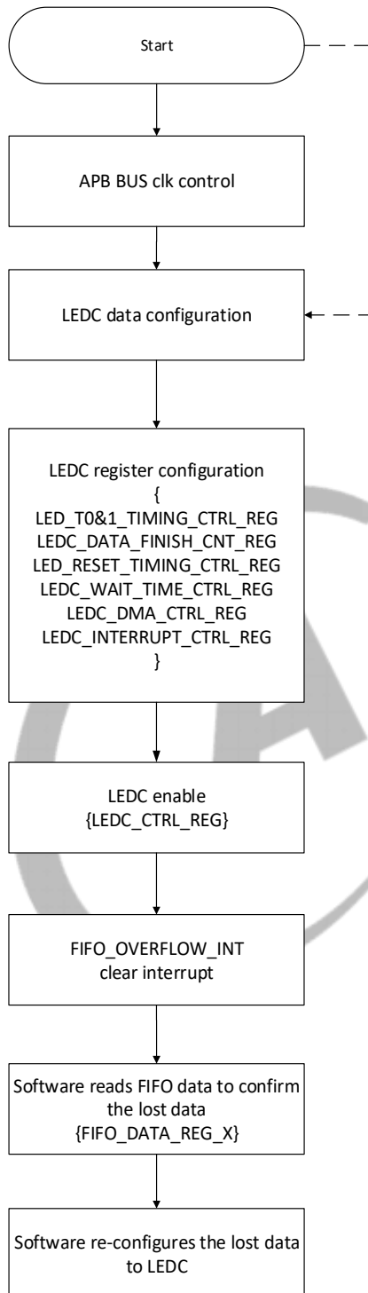
Figure 9-102 FIFO Overflow Abnormal Processing Flow
