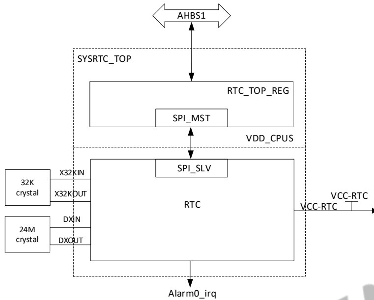
Figure 3-35 RTC Application Diagram
