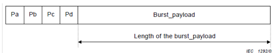
Figure 8-22 Length of the Burst-Payload Specified by Pd
