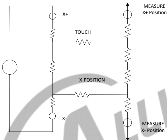
Figure 9-76 Dual Touch Detection for Touch Panel
