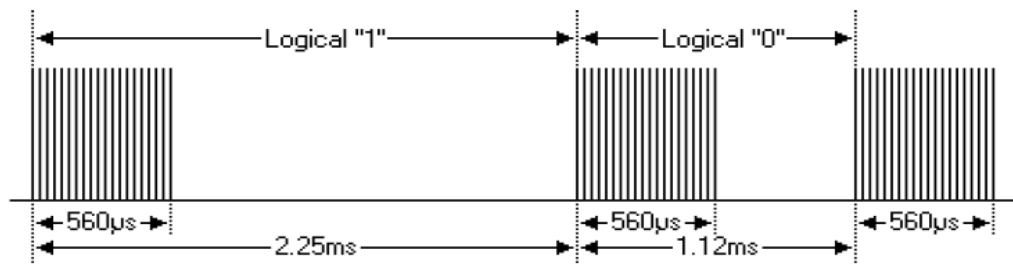
Figure 9-118 Definitions of Logical "1" and Logical "0"
