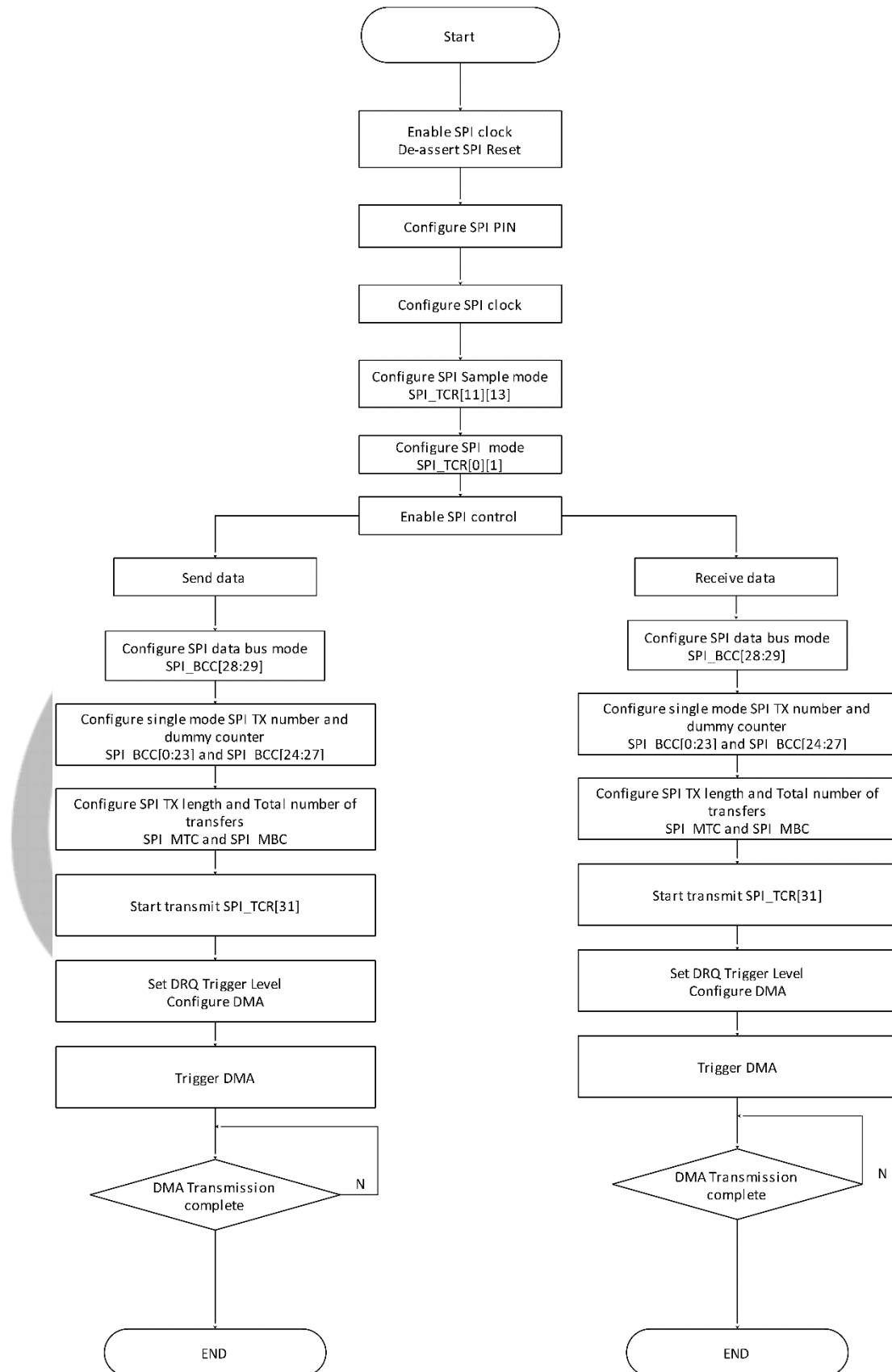
Figure 9-62 SPI Write/Read Data in DMA Mode
