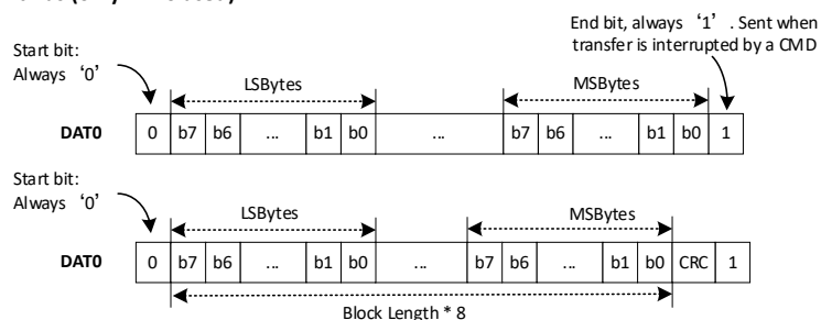
Figure 7-4 Data Packet Format for SDR
