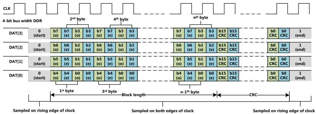
Figure 6-4 Timing for 4-bit DDR Mode
