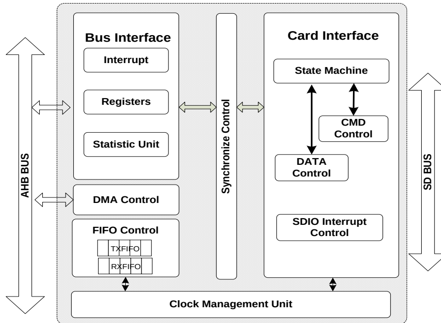
Figure 6-1 SD Host Controller Block Diagram
