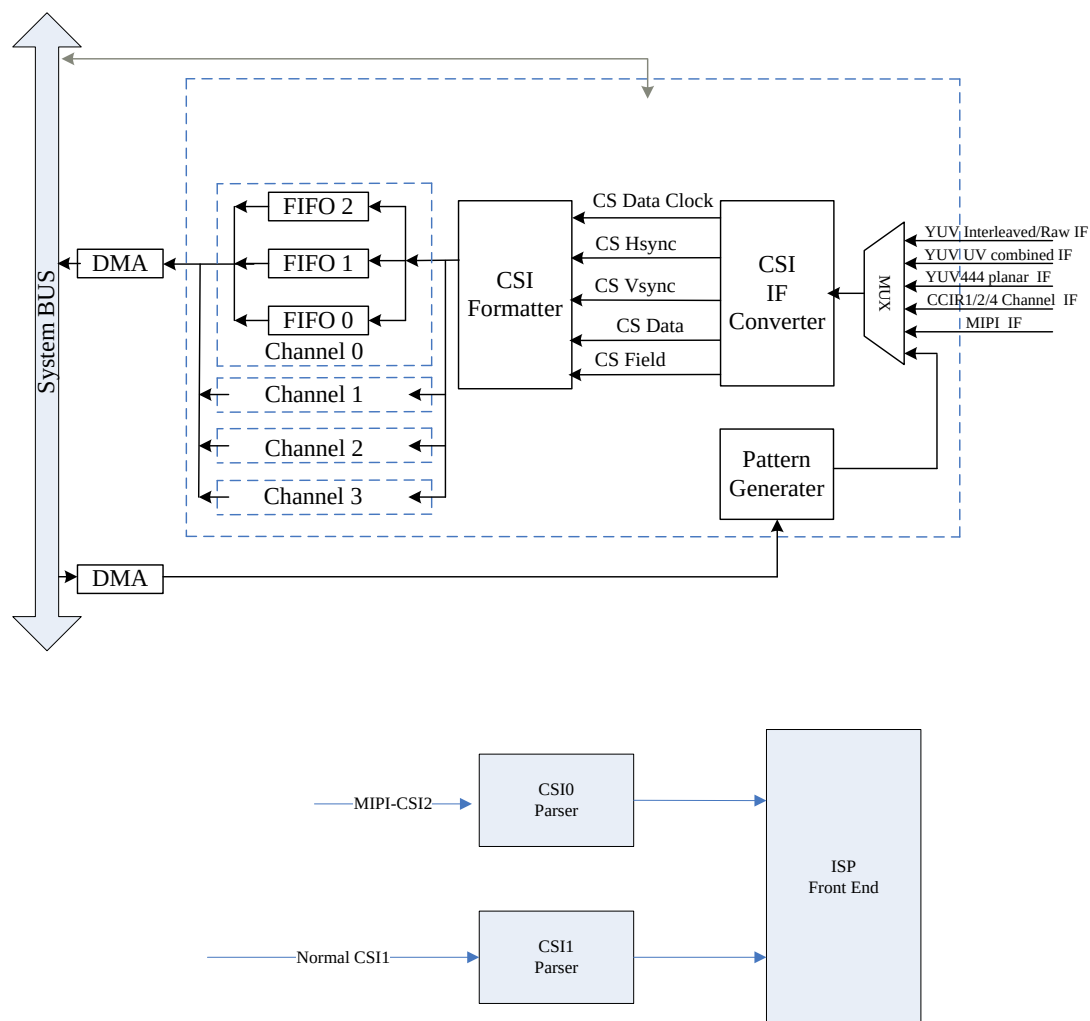
Figure 4-2 CSI1 Block Diagram
