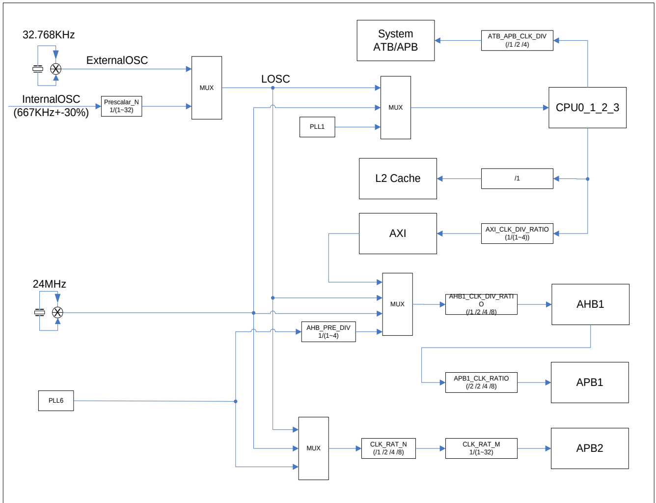
Figure 1-3 CPU Clock Diagram
