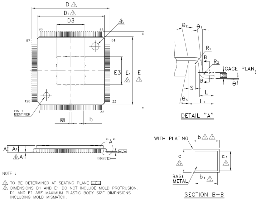
Figure 7-2 D1s Package Dimension
