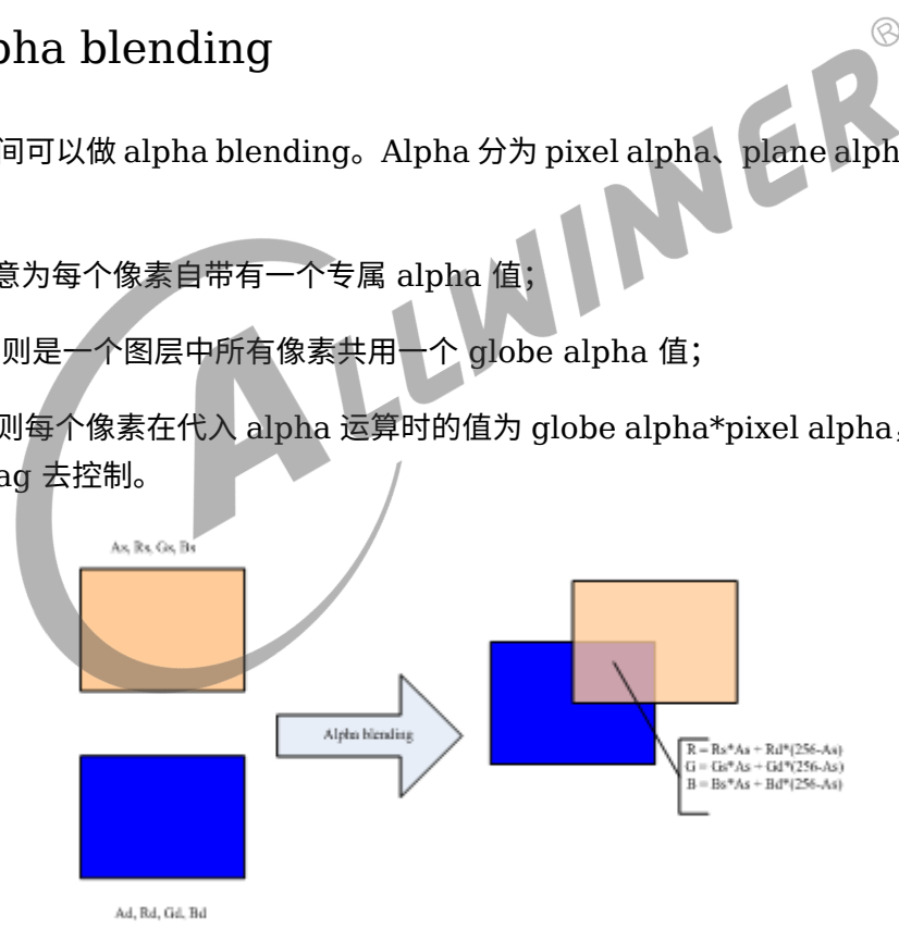
图 2-3: alpha blending 1
