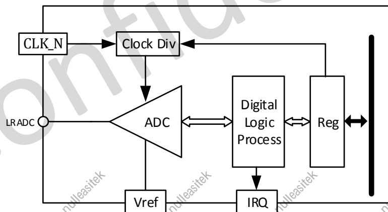
Figure 9- 35. LRADC Block Diagram
