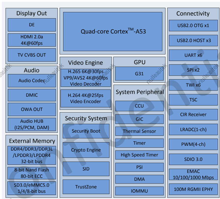
Figure 2- 1. H616 System Block Diagram
