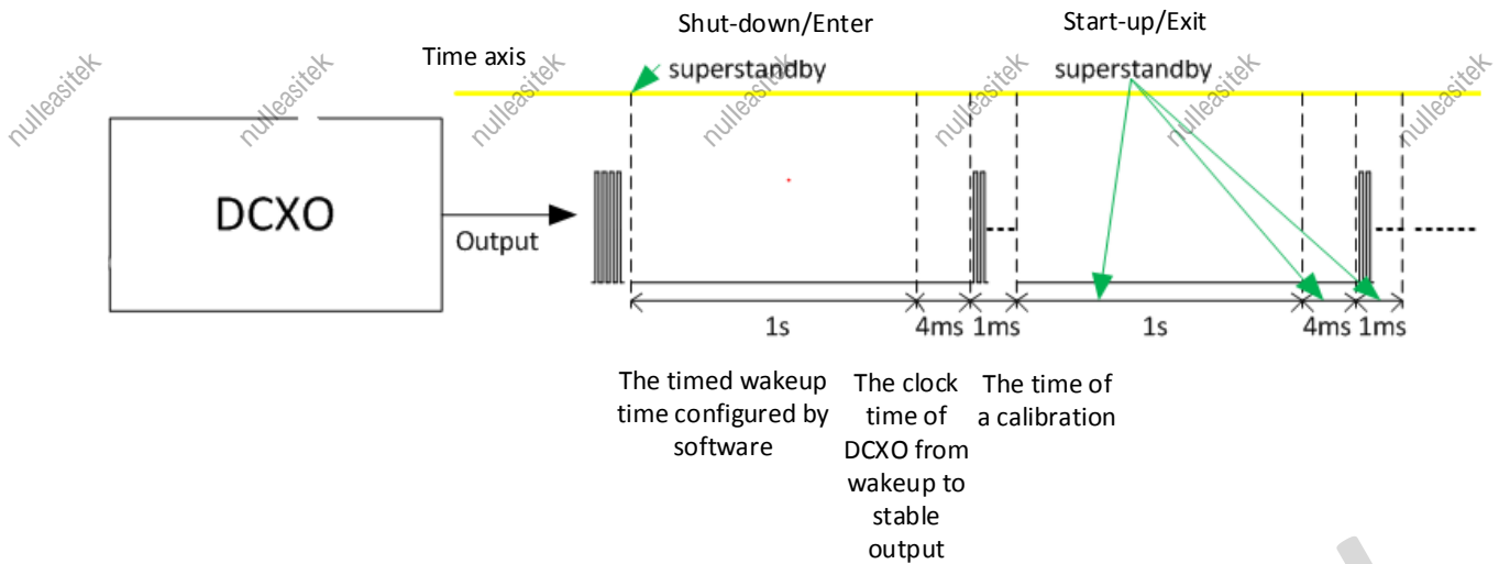
Figure 3- 41. DCXO Timed Wakeup Waveform
