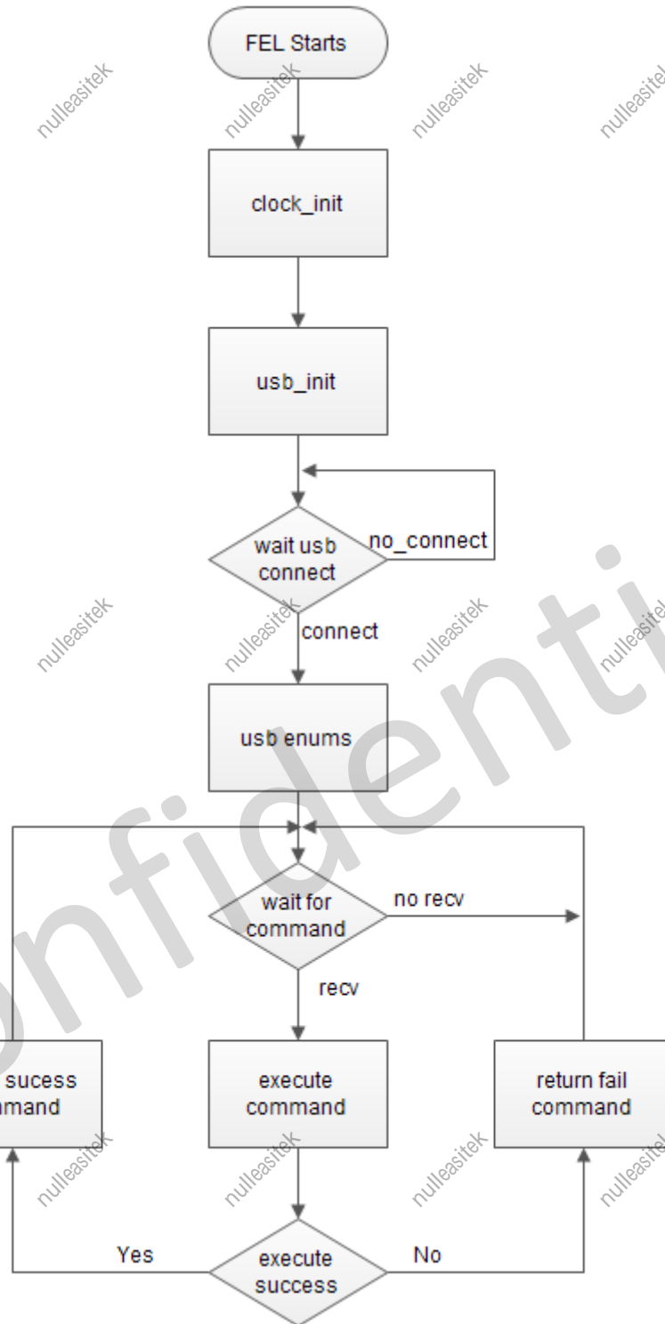
Figure 3- 9. USB FEL Process
