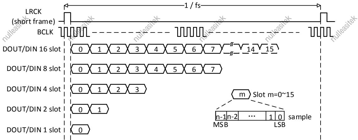
Figure 8- 8. Timing Diagram for PCM Mode (short frame)
