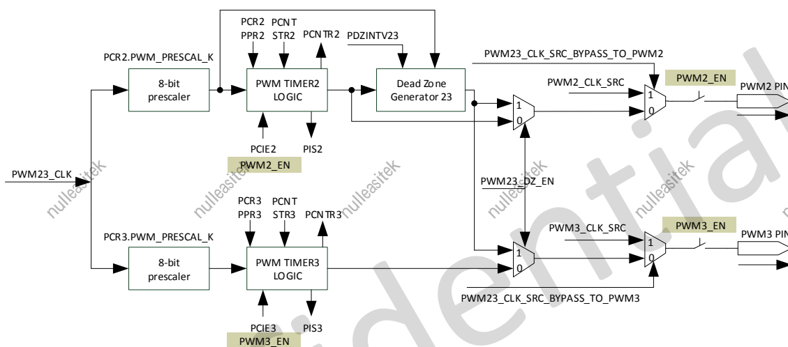
Figure 9- 50. PWM23 Pair Output Logic Module Diagram
