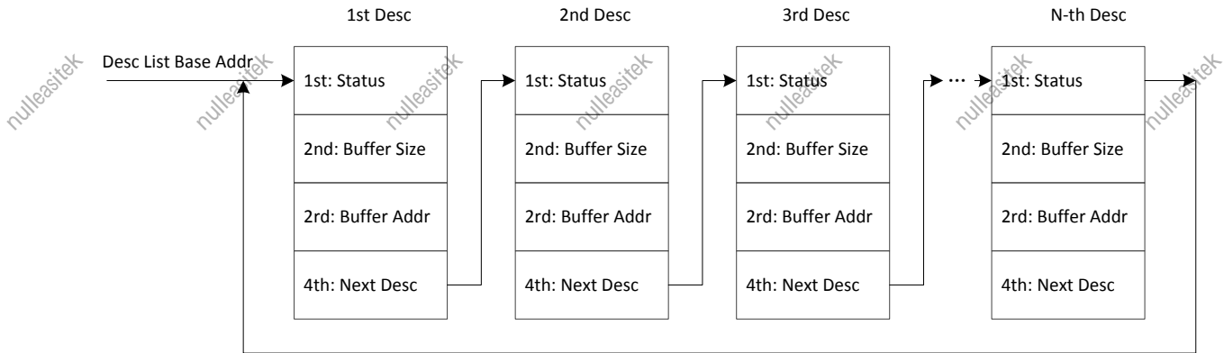
Figure 6- 3. EMAC RX/TX Descriptor List
