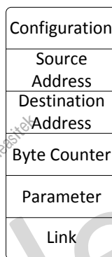
Figure 3- 19. DMA Descriptor
