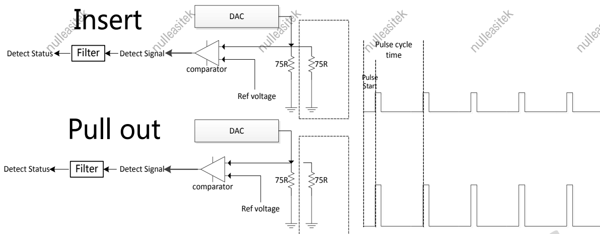
Figure 7- 9. Auto Detect Function
