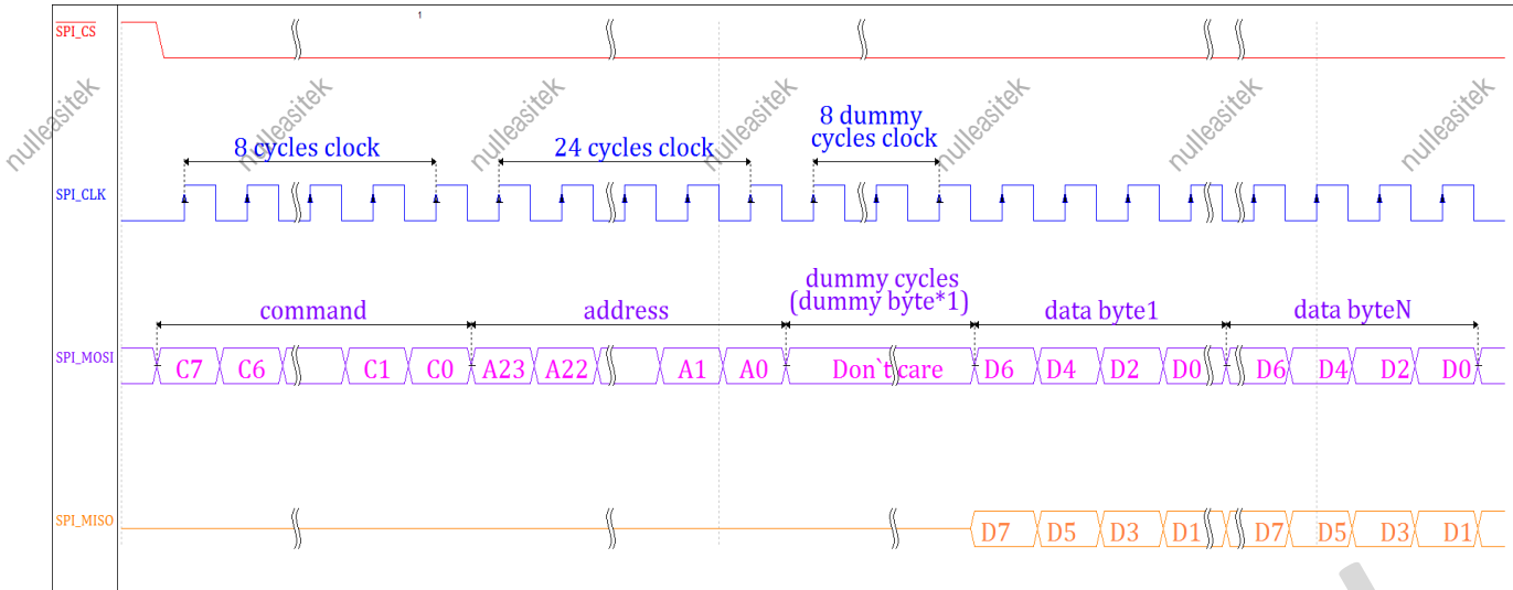
Figure 9- 24. SPI Dual-Input/Dual-Output Mode
