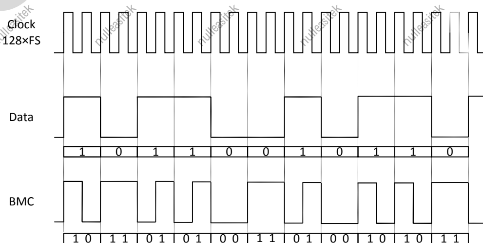
Figure 8- 15. OWA Biphase-Mark Code
