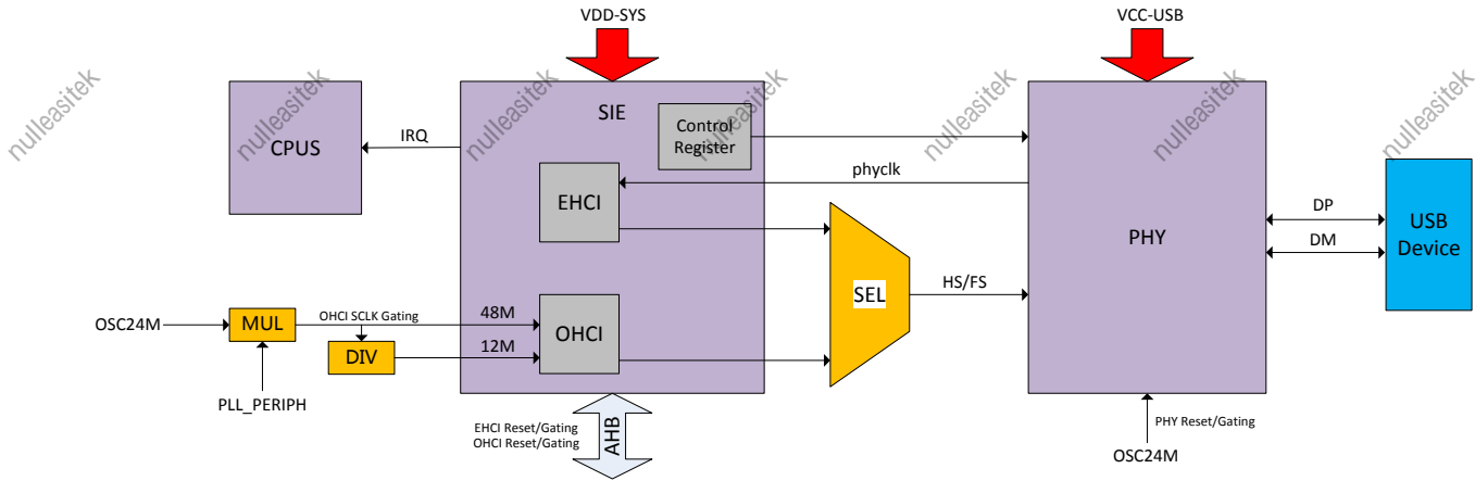
Figure 9- 31. USB2.0 HOST Controller and PHY Connection Diagram
