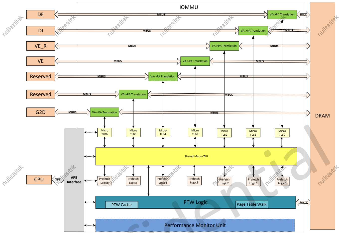
Figure 3- 28. IOMMU Block Diagram
