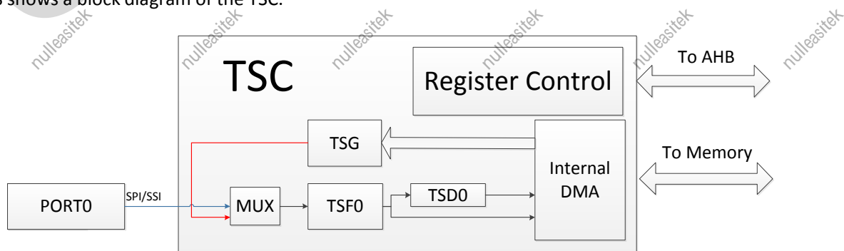
Figure 9- 58. TSC Block Diagram
