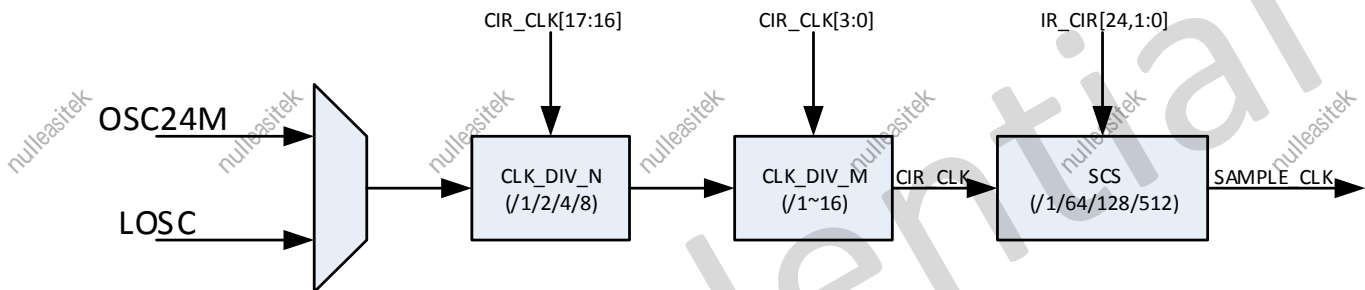
Figure 9- 39. CIR Receiver Clock
