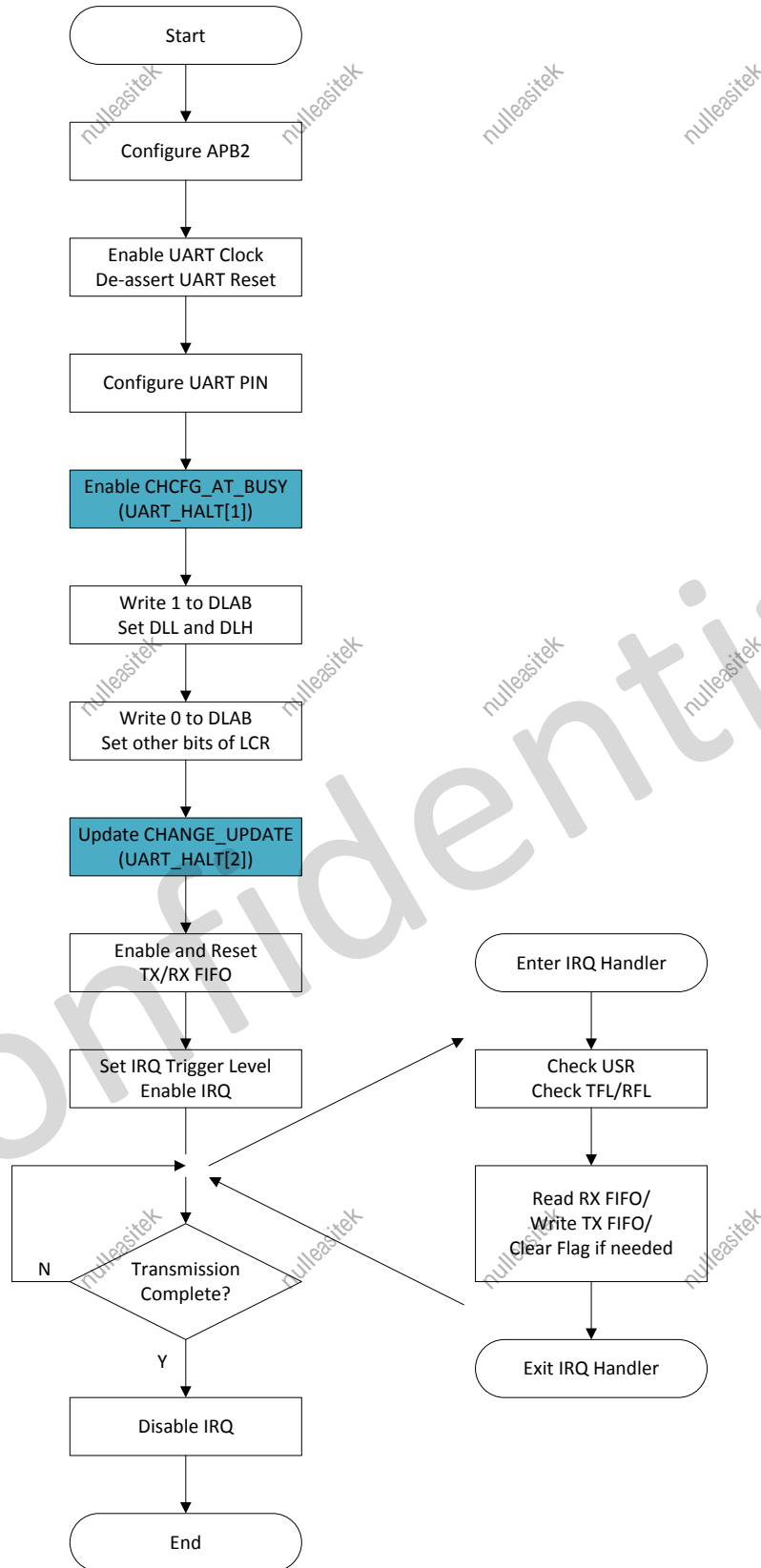
Figure 9- 17. Process of UART Transmitting/Receiving Data in Interrupt Mode
