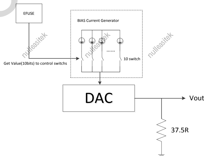
Figure 7- 10. DAC Calibration
