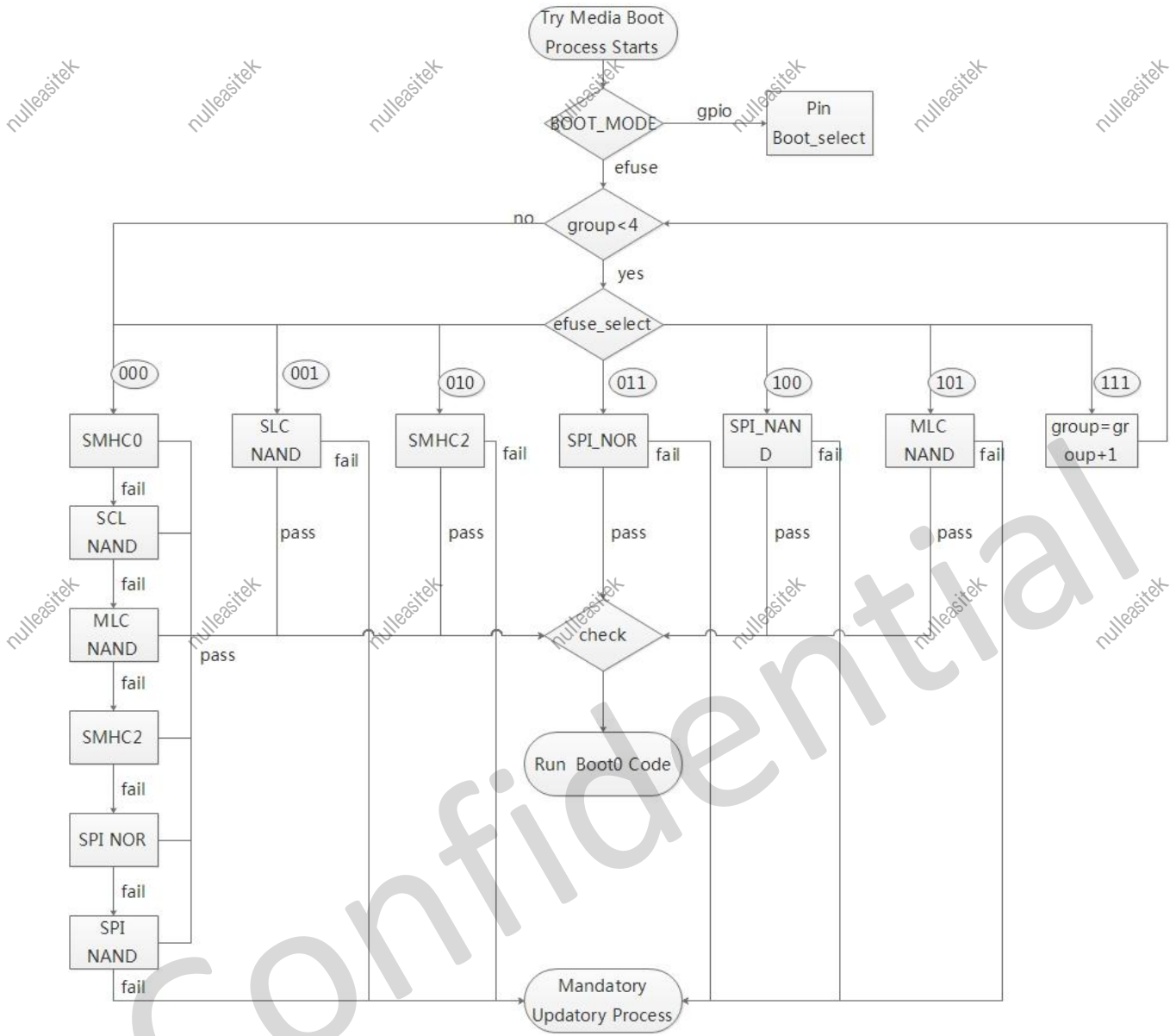
Figure 3- 11. eFuse Boot Select Process
