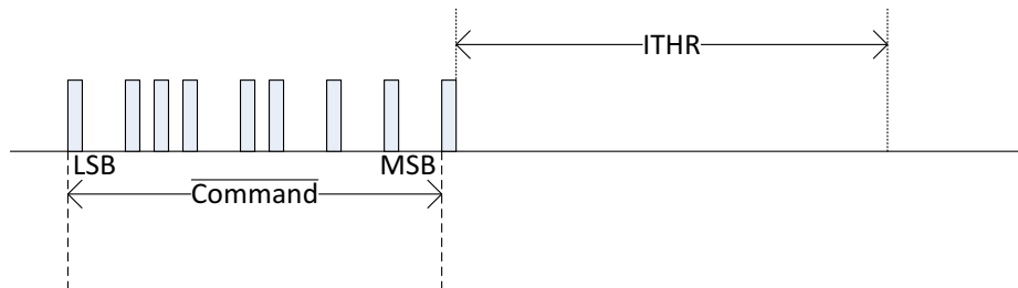
Figure 10- 48. ITHR Definition
