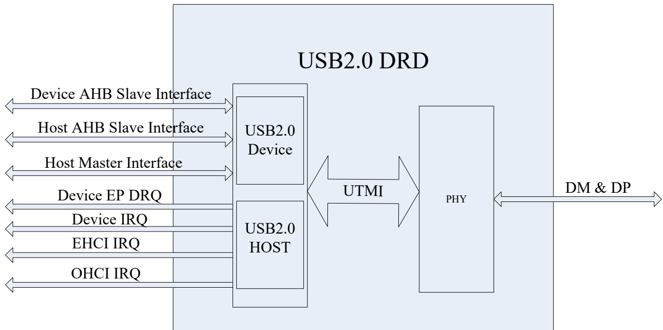
Figure 10- 29. USB2.0 OTG Controller Block Diagram
