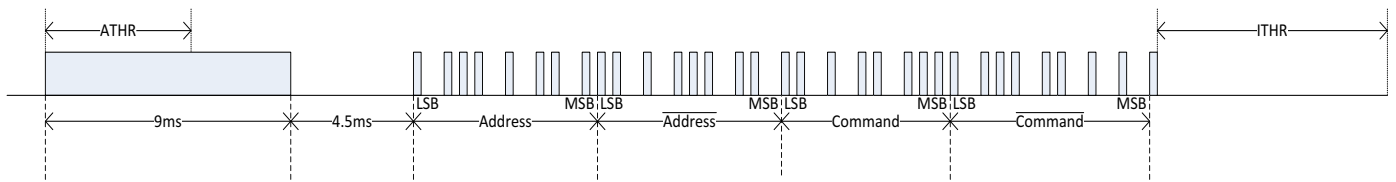
Figure 10- 45. NEC Protocol
