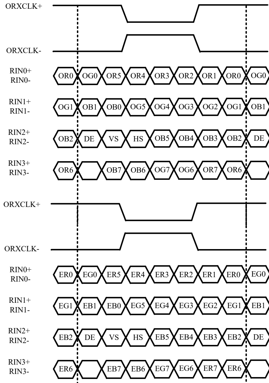
Figure 6- 7. LVDS Dual Link NS Mode Interface Timing
