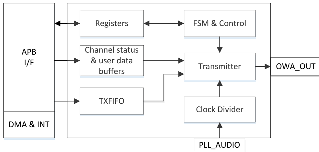
Figure 9- 11. OWA Block Diagram
