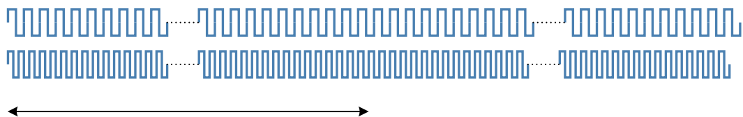
Figure 3- 36. RC Waveform
