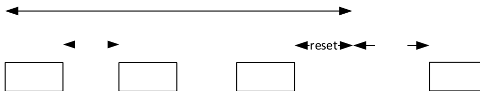
Figure 10- 71. LEDC 1-frame Output Timing Diagram
