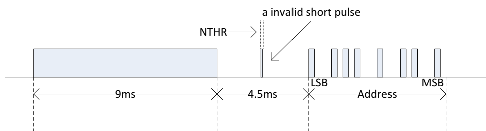
Figure 10- 49. NTHR Definition
