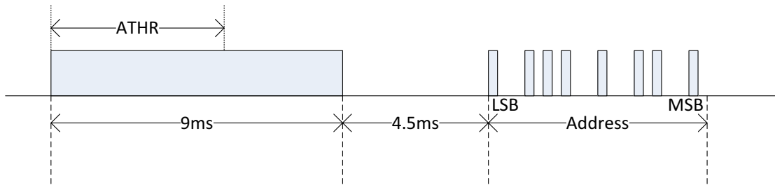
Figure 10- 47. ATHR Definition
