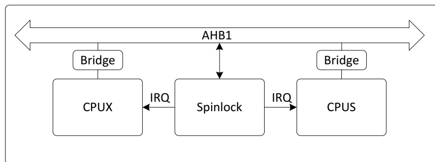
Figure 3- 41. Spinlock Block Diagram
