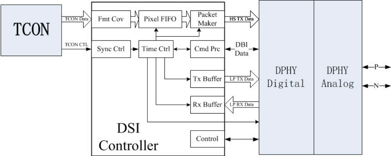
Figure 6- 15. MIPI DSI Internal Unit
