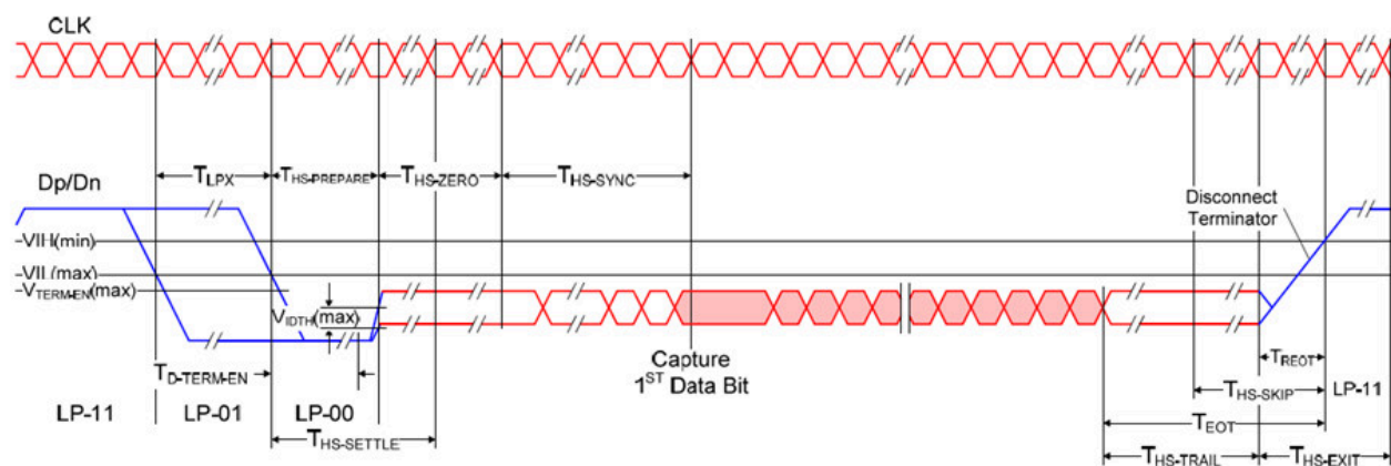
Figure 6- 18. DPHY SOT and EOT Timing
