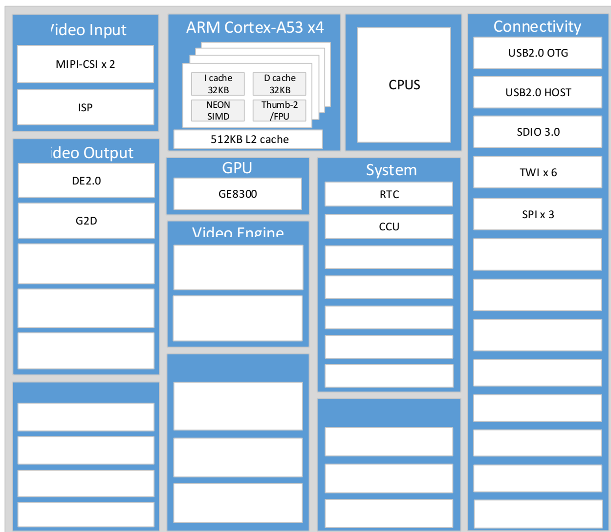
Figure 2- 1. R818 System Block Diagram
