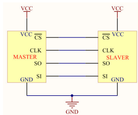
Figure 10- 20. SPI Application Block Diagram
