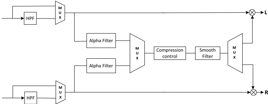
Figure 9- 24. DAP Data Flow
