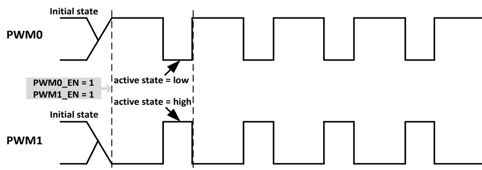
Figure 10- 64. PWM01 Complementary Pair Output
