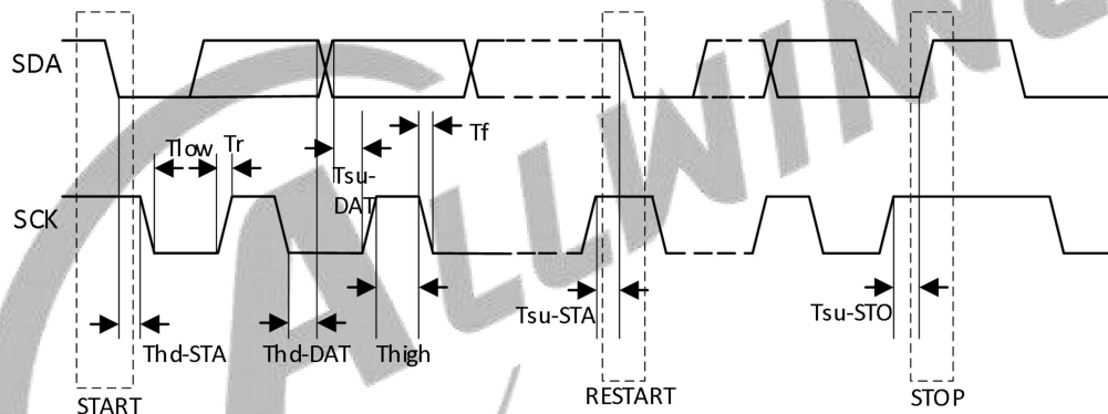
Figure 6-30 TWI Timing
