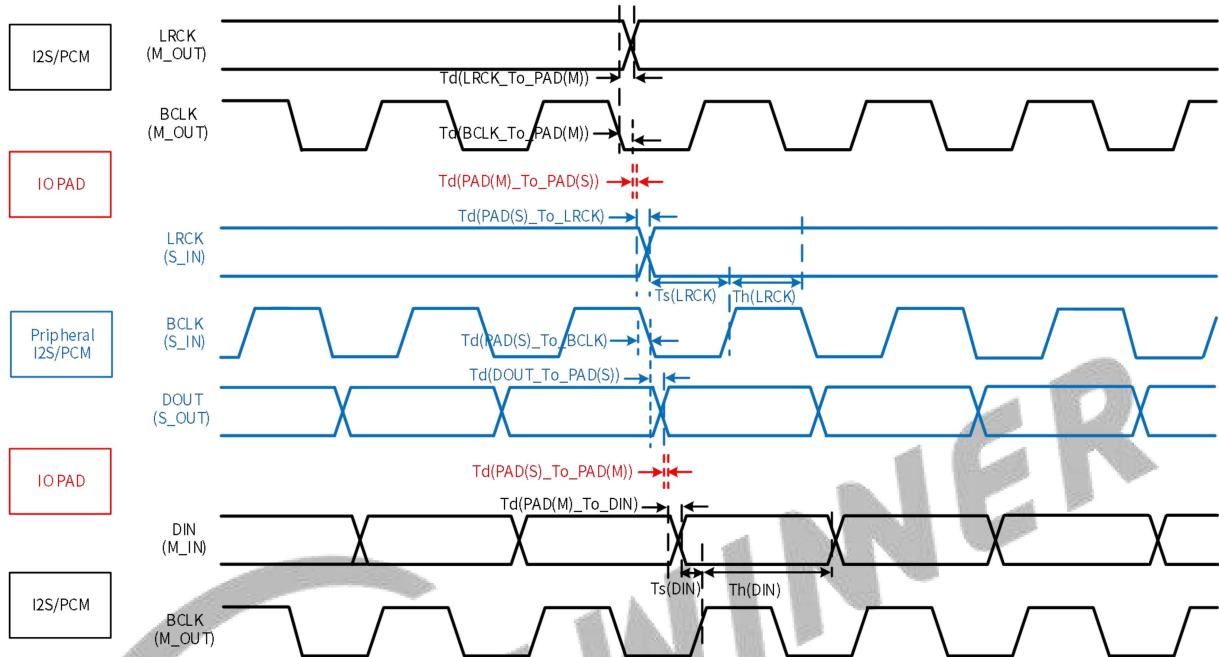
Figure 6-37 Data Input Timing of I2S/PCM in Master Mode
