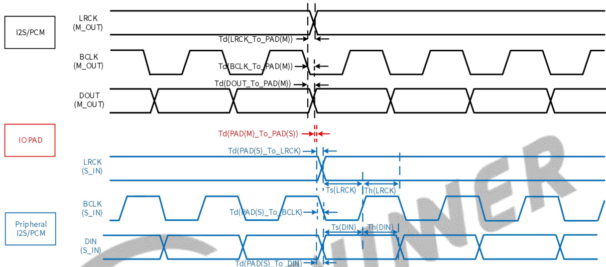
Figure 6-36 Data Output Timing of I2S/PCM in Master Mode
