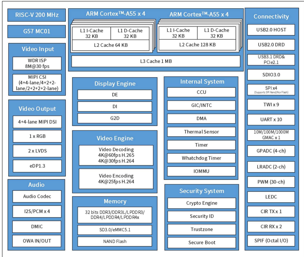
Figure 4-1 A523 System Block Diagram
