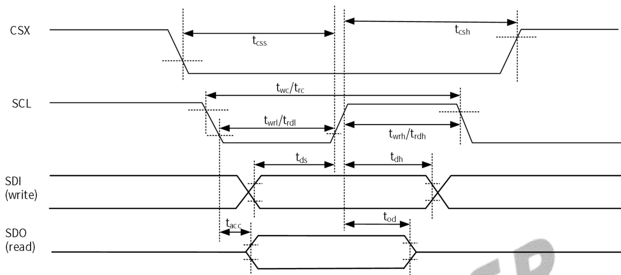
Figure 6-26 DBI 3-line Serial Interface Timing
