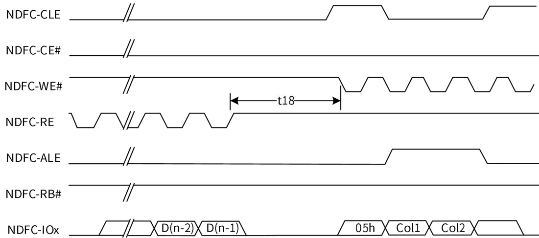
Figure 6-12 Address to Data Loading Timing
