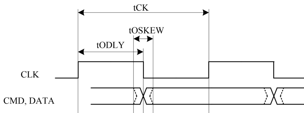
Figure 6-13 SMHC HS-SDR Mode Output Timing Diagram
