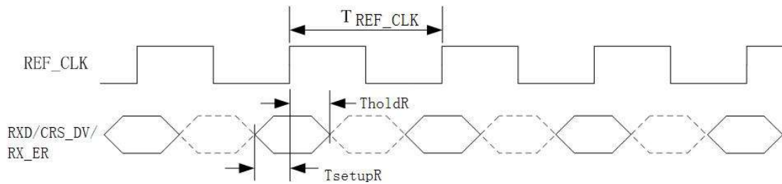
Figure 6-34 RMII Transmit Timing
