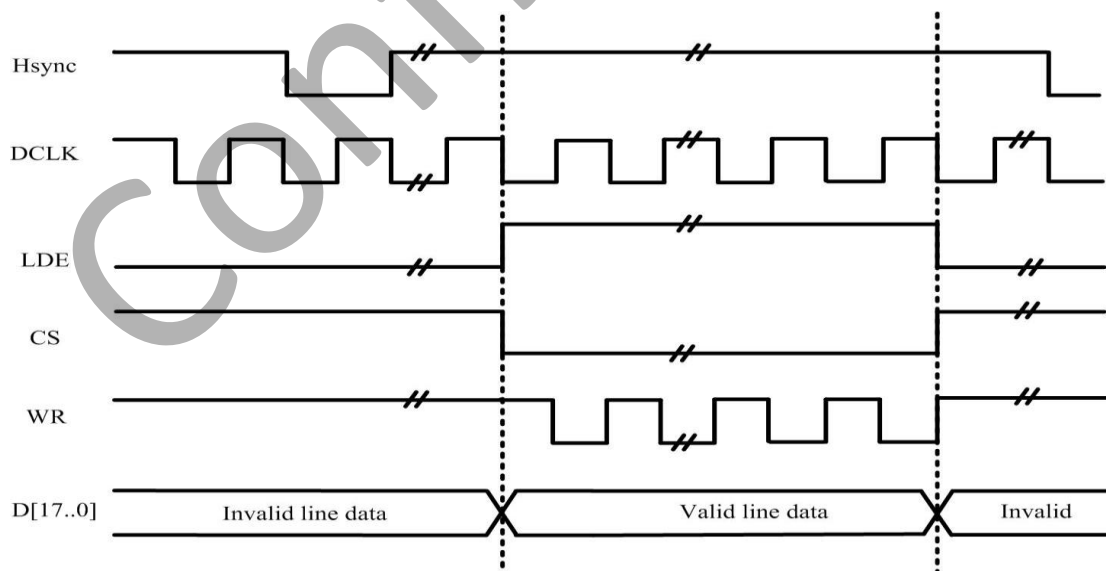
Figure 6-8. Lcd_CPUI/F Timing
