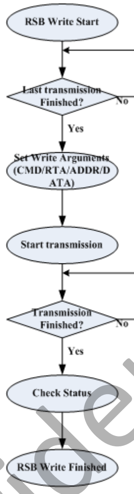
Figure 7-6. RSB Write to Device
