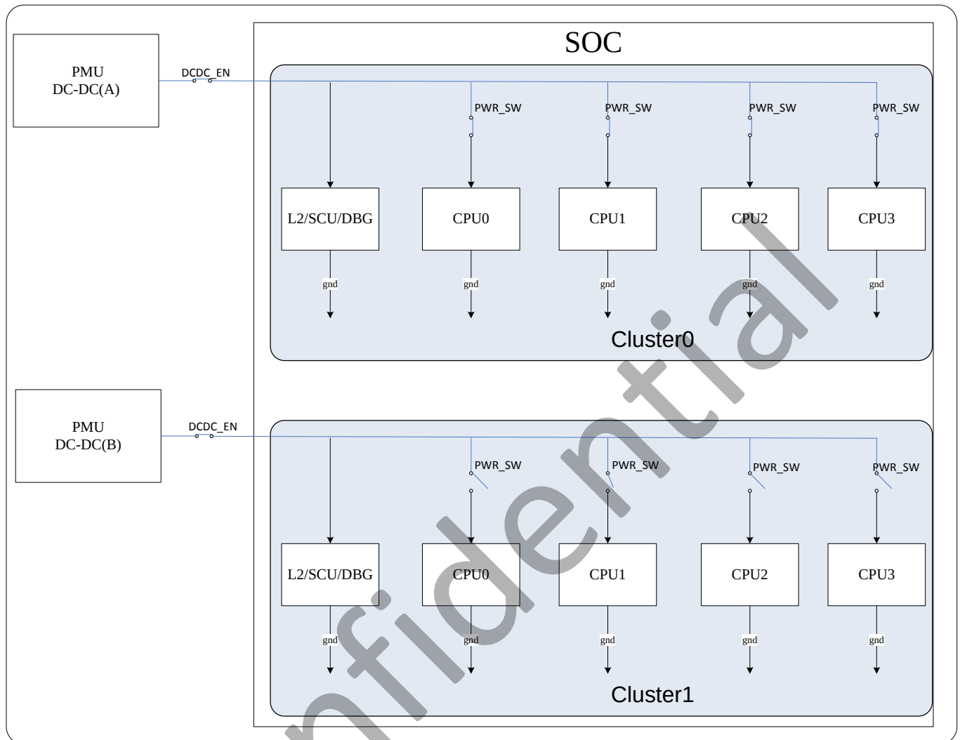
Figure 3-3. CPU Power Domain Diagram(Default State)
