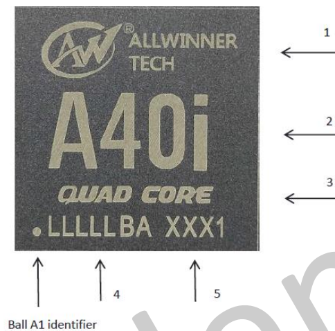
Figure 12-1. A40i Marking
