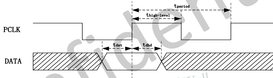
Figure 5-28. 8-bit YCbCr4:2:2 with Embedded Syncs(BT656) Timing
