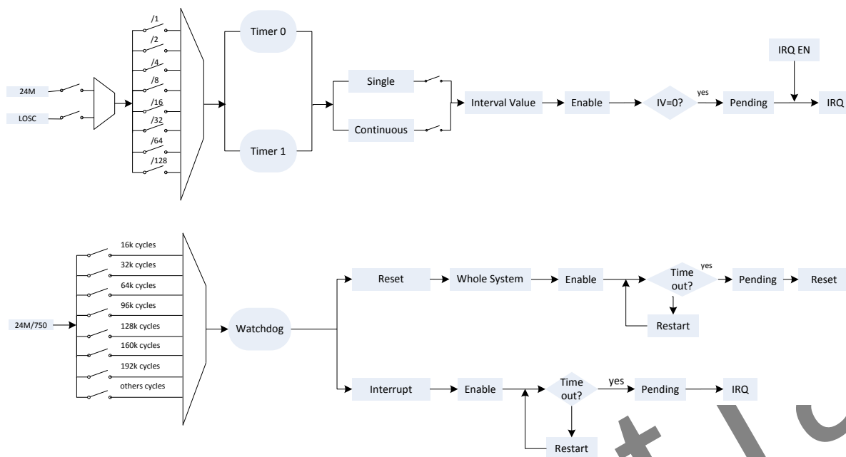
Figure3.5-1 Timer Block Diagram
