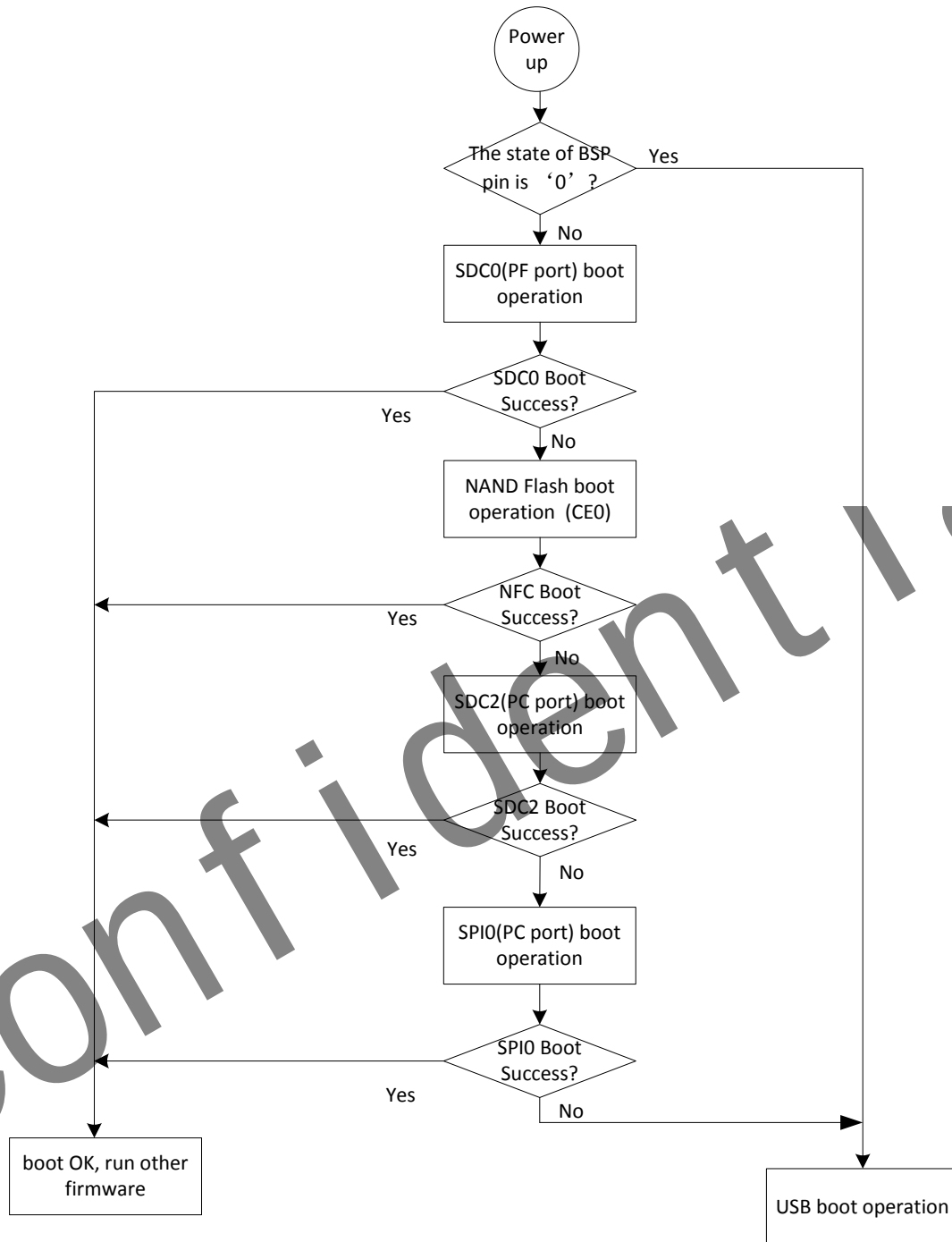
Figure 3.2-1 Boot Diagram
