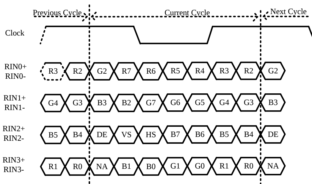
Figure 5.2-4 Single channel: JEDIA mode
