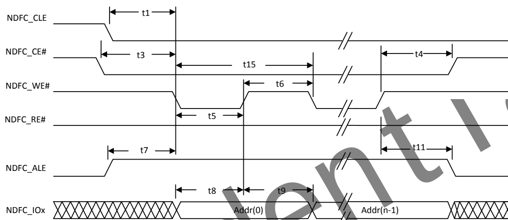
Figure4.2-6 Address Latch Cycle
