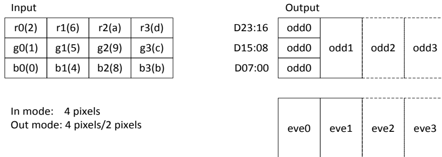
Figure 5.2-6 CMAP Module
