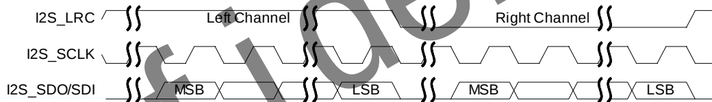
Right-justified I2S Timing Diagram
