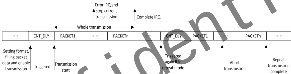
Figure 6.1-7 transmission process
