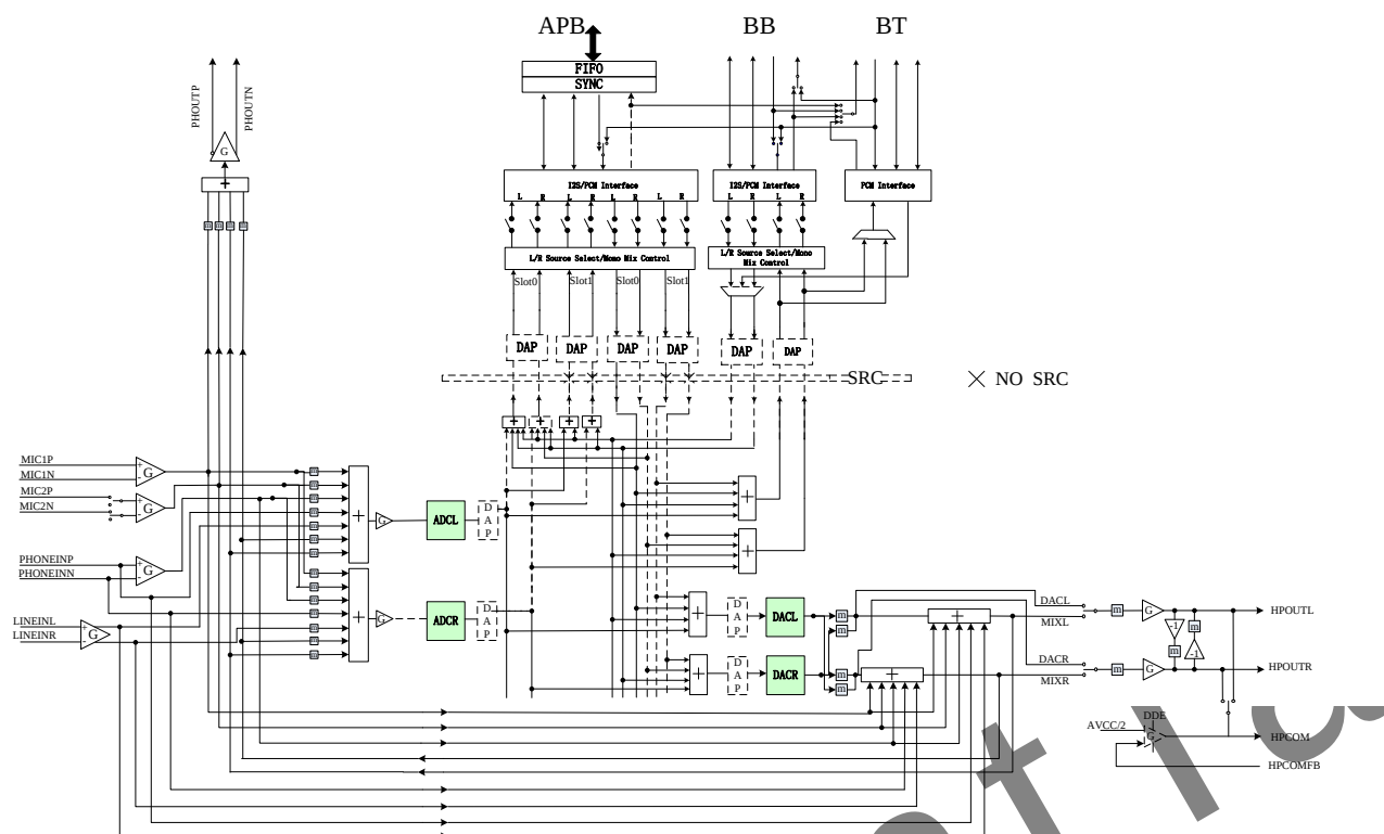
Figure 3.16-1 Audio CODEC Block Diagram
