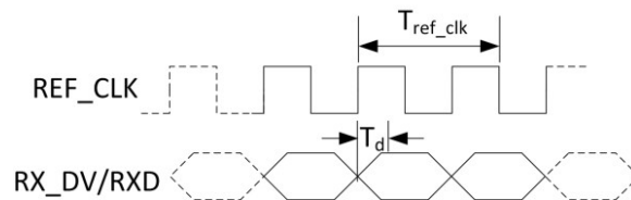
Figure 5-41. RMII Interface Receive Timing
