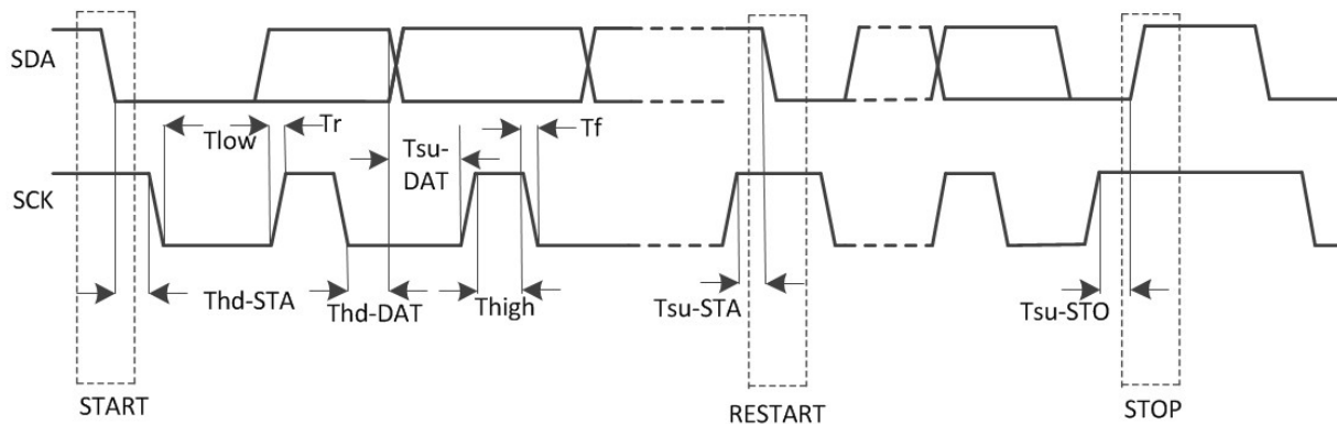
Figure 5-50. TWI Timing
