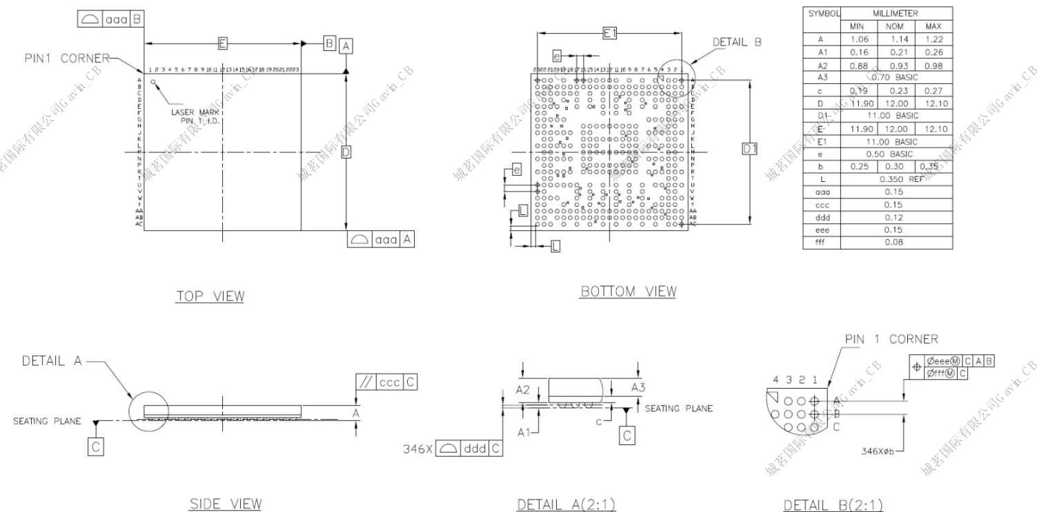
Figure 7-2. R818 Package Dimension
