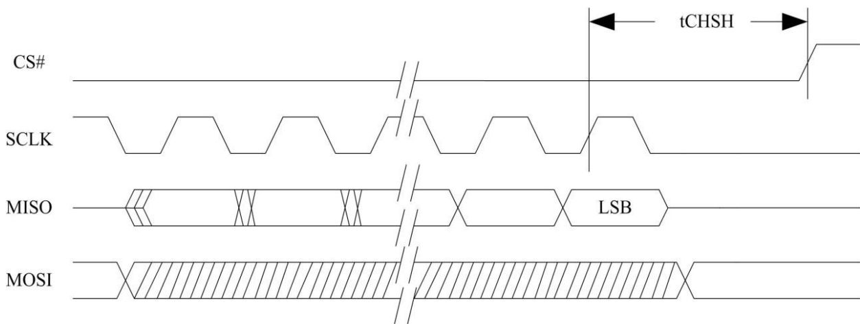
Figure 5-46. SPI MISO Timing
