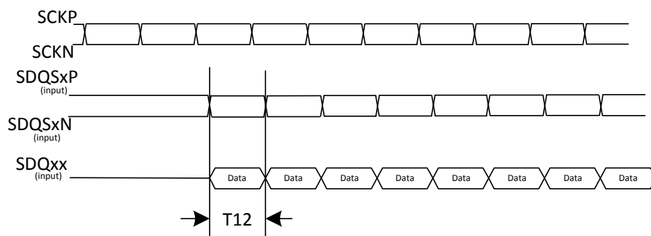
Figure 5-7. LPDDR3 Read Cycle
