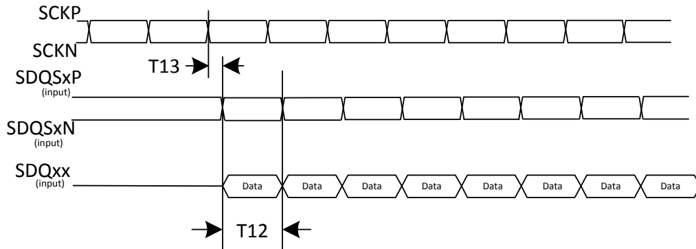
Figure 5-4. DDR3/DDR3L Read Cycle
