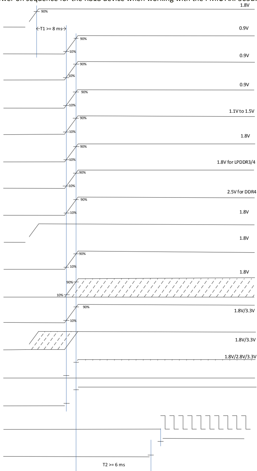
Figure 5-55. R818 Power On Sequence (with AXP305B)
