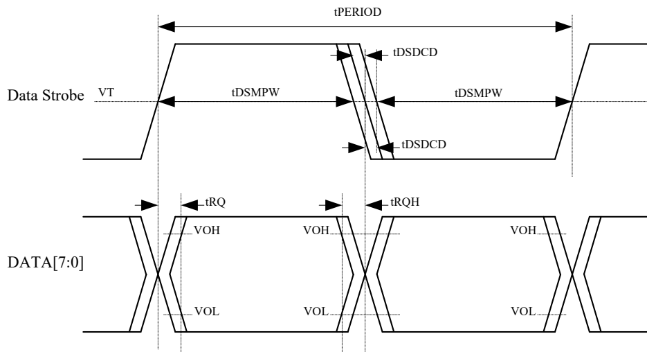
Figure 5-37. SMHC2 HS400 Mode Data Input Timing Diagram
