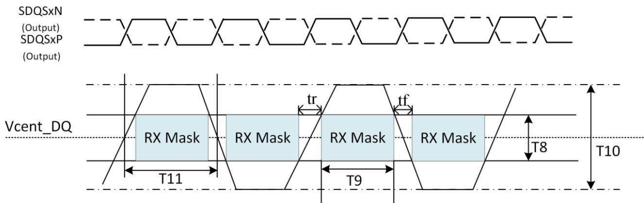
Figure 5-12. LPDDR4 Write Cycle
