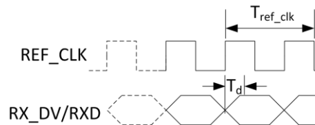
Figure 5-41. RMII Interface Receive Timing
