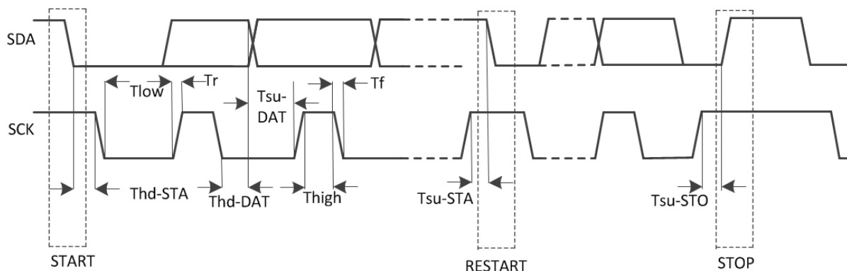
Figure 5-50. TWI Timing
